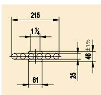
Retro 6 Column Depth 215mm Wall to Front Edge 250mm Wall to Pipework centre 143mm
