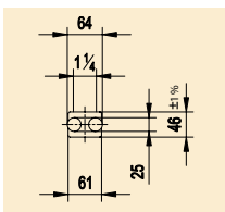
Retro 2 Column Depth 64mm Wall to Front Edge 99mm Wall to Pipework centre 67mm
